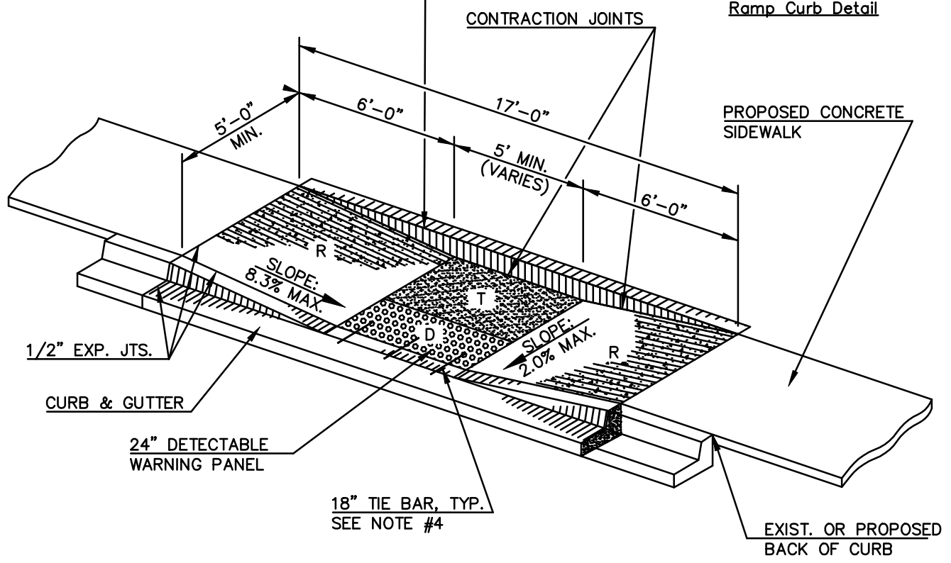
TYPE IV SIDEWALK RAMP
