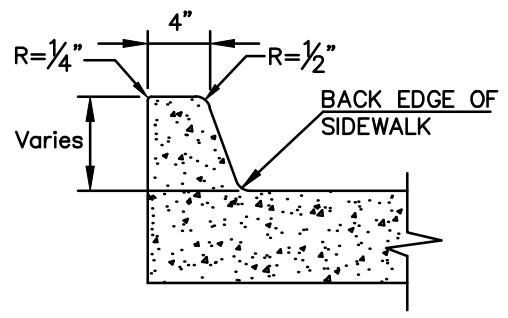
Ramp Curb Detail
