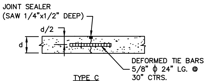
TYPE C TIED BUTT LONGITUDINAL CONSTRUCTION JOINT
