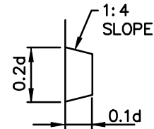
KEYWAYS FOR TYPE B AND F CONSTRUCTION JOINT
