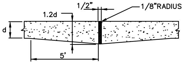
TYPE A EXPANSION JOINT
