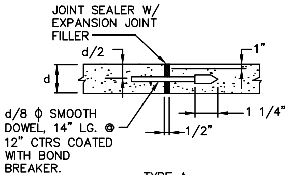
TYPE A ALTERNATE EXPANSION JOINT
