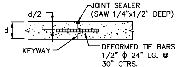
TYPE F EMERGENCY TIED TRANSVERSE CONSTRUCTION JOINT
