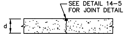
TYPE D SAWED LONGITUDINAL OR TRANSVERSE
