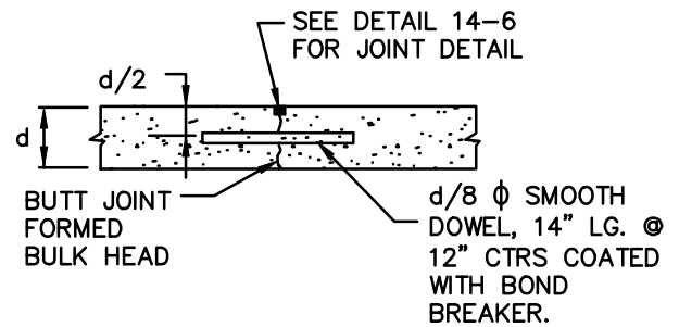
TYPE E PLANNED TRANSVERSE CONSTRUCTION JOINT (USED AT NORMAL JOINT SPACING)
