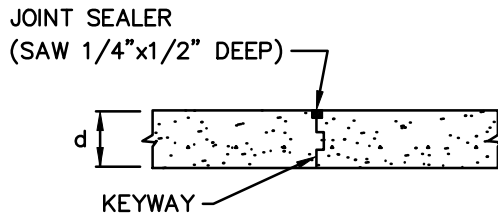
TYPE B LONGITUDINAL CONSTRUCTION JOINT
