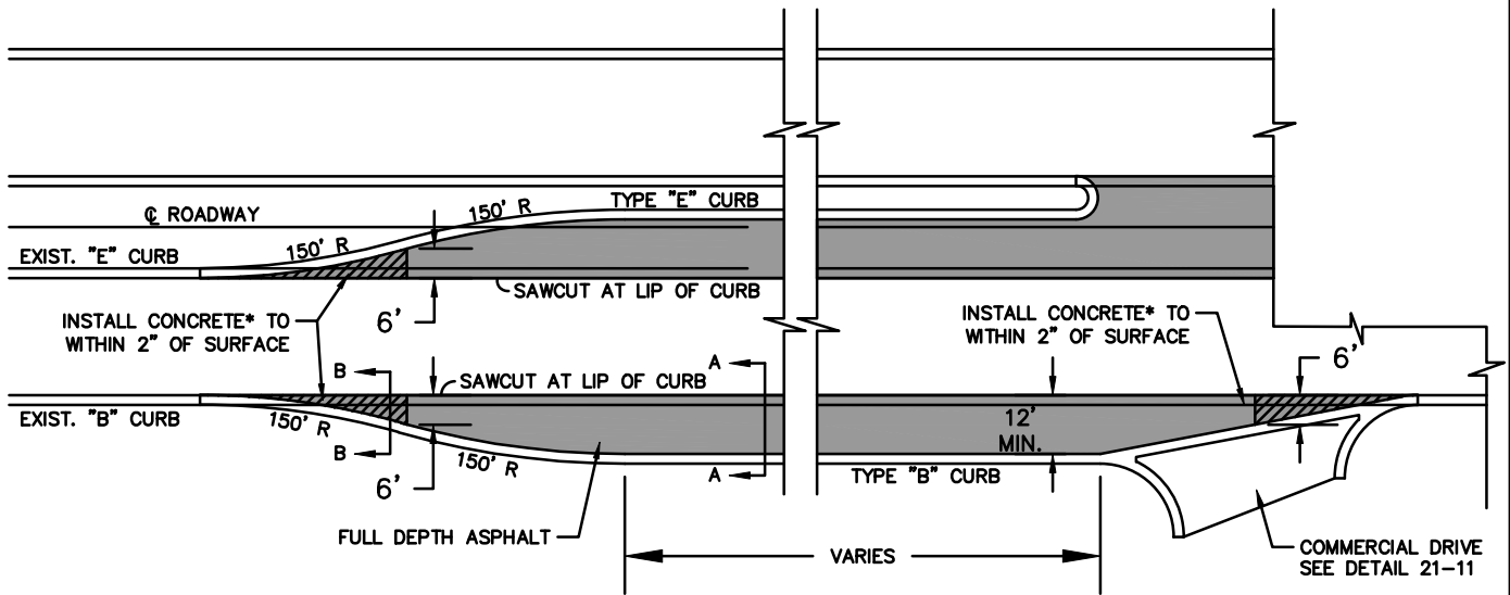
TYPICAL LANE WIDENING N.T.S.
